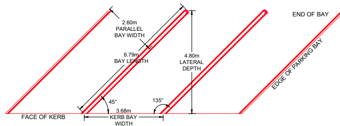
45° PARKING BAY MEASUREMENTS TAKEN FROM AS2890.5:2020
