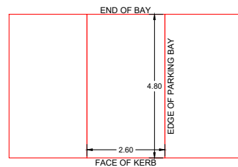
90° PARKING BAY MEASUREMENTS TAKEN FROM AS2890.5:2020
